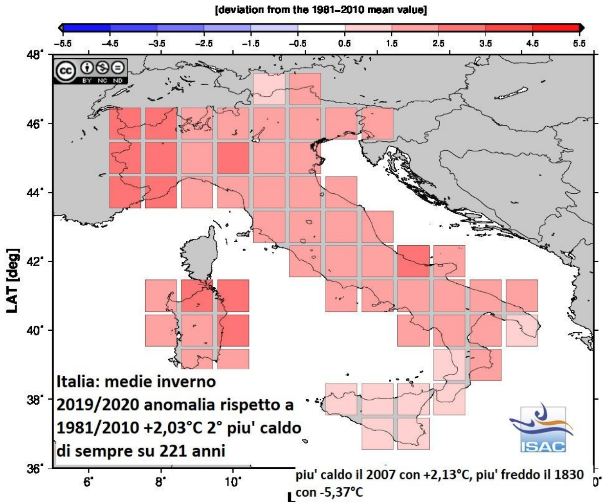
Fig. 1: temperature medie Italia inverno 2019/2020
